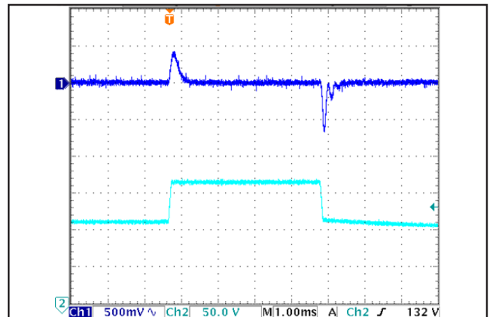
Figure 6: Output voltage response to step-change in input voltage (1V/ms). Load cap: 1 \mu F ceramic capacitor. Ch 1: V_{out} , Ch 2: V_{in} .
