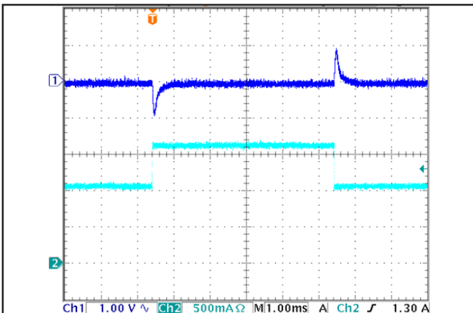
Figure 5: Output voltage response to step-change in load current (50%-75%-50% of I_{out(max)} ; dI/dt = 0.1 A/\mu s ). Load cap: 1 \mu F ceramic capacitor. Ch 1: V_{out} , Ch 2: I_{out} (500mA/div)
