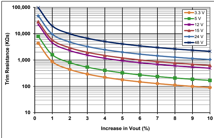
Common Figure 3: Trim graph for trim-up 3.3 to 48V outputs.
